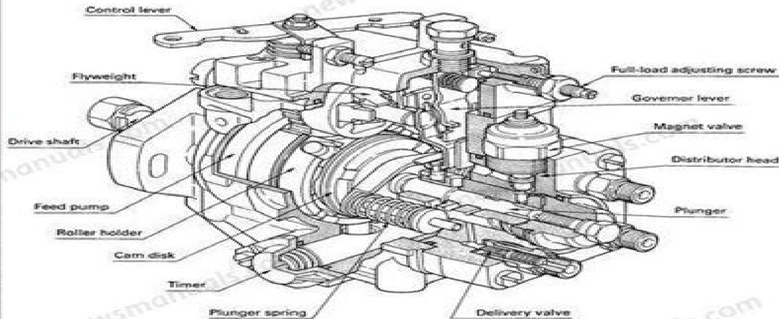
Fig. 1 VE type injection pump construction
