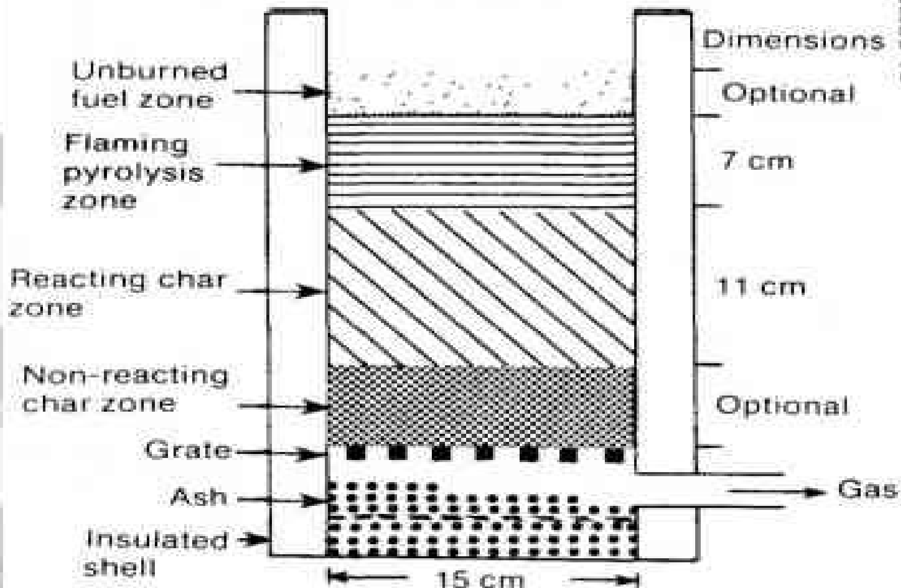
Fig. 5-13. Stratified downdraft gasifier design (Source: Reed 1984, Fig. 6)
