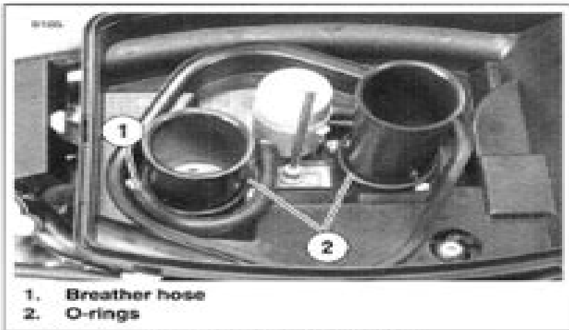
Figure 1-4. Velocity Stacks
