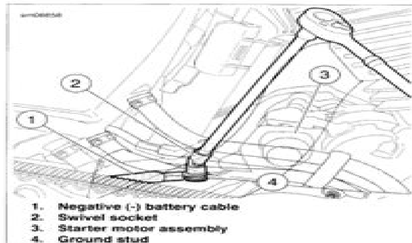
Figure 1-66. Negative (-) Battery Connection
