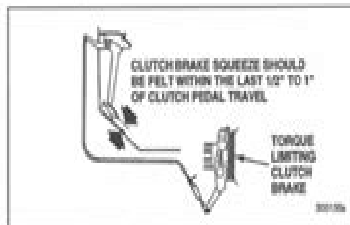
Figure 88 — Clutch Brake Squeeze (Spicer Easy Pedal)
