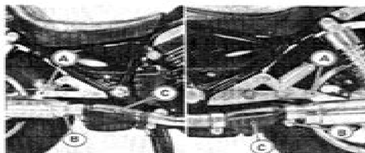
A. Mounting Bolt and Nut B. Clamp Bolt C. Power Chamber
