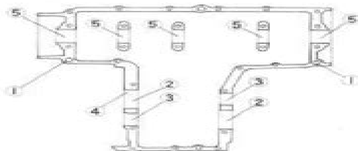
1. Knock pins 2. Set rings 3. Set pins 4. Rubber oil passage plug 5. Main bearing inserts
