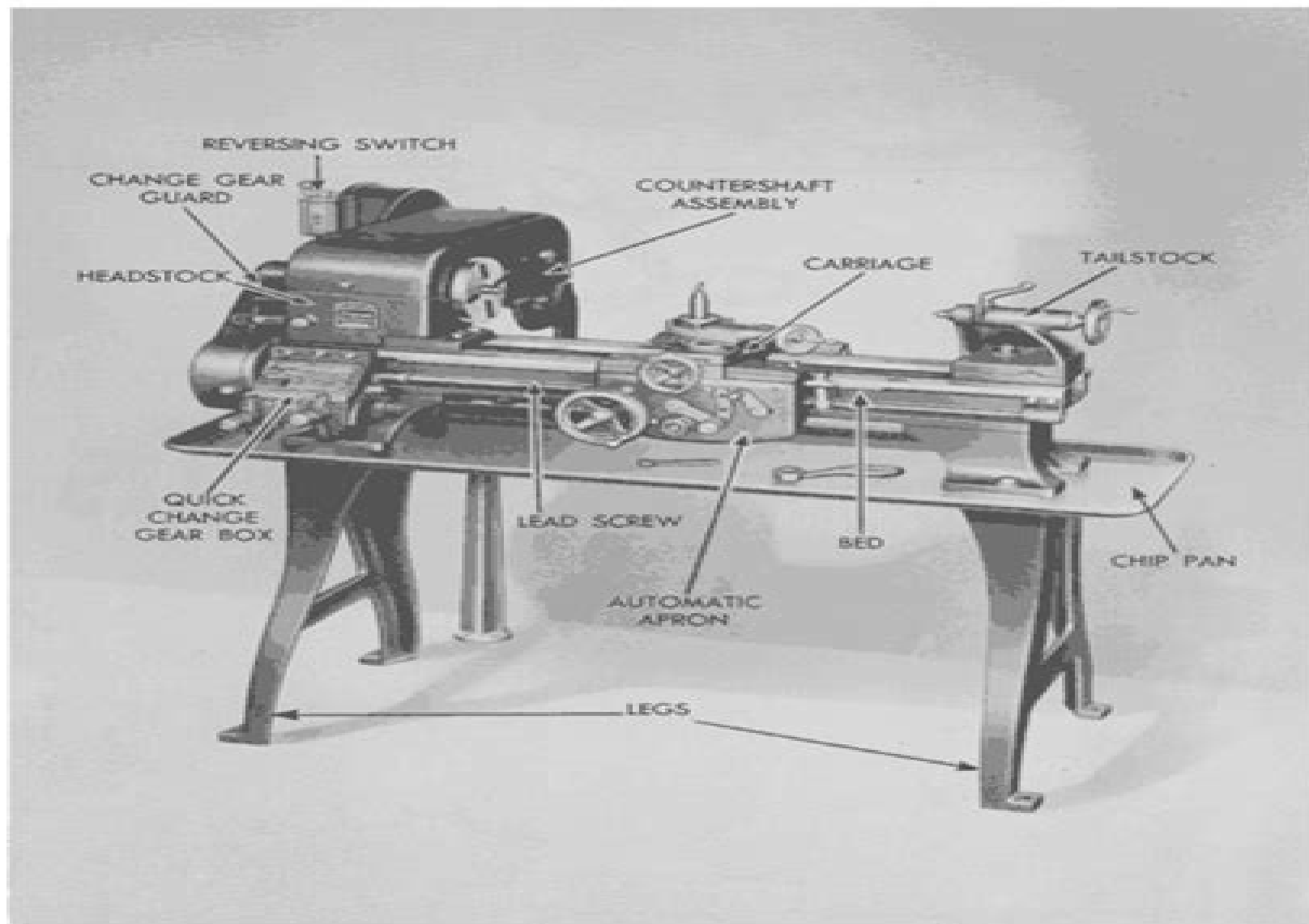
FIGURE 1—LOGAN NO. 825 FLOOR MODEL QUICK CHANGE GEAR LATHE
