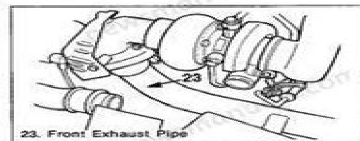
Figure 10. Exhaust Pipe Attachment
