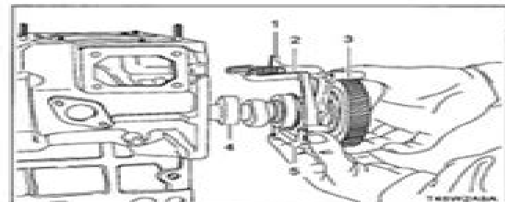
(1) Fork Lever 1
