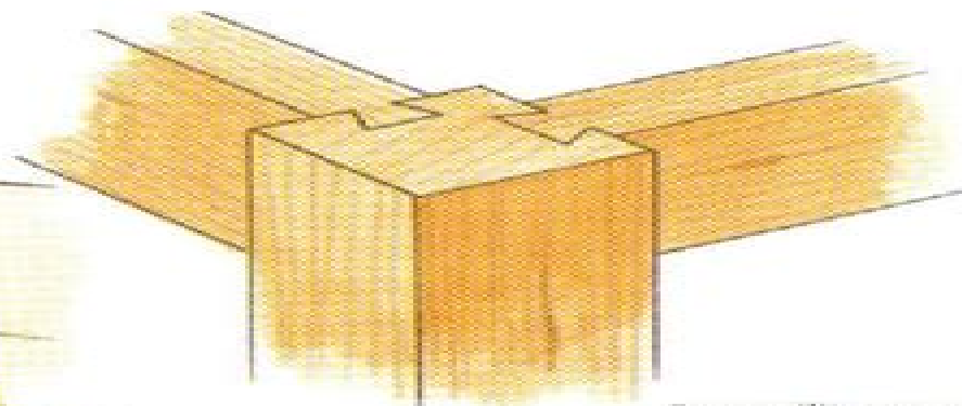
Sliding dovetail
