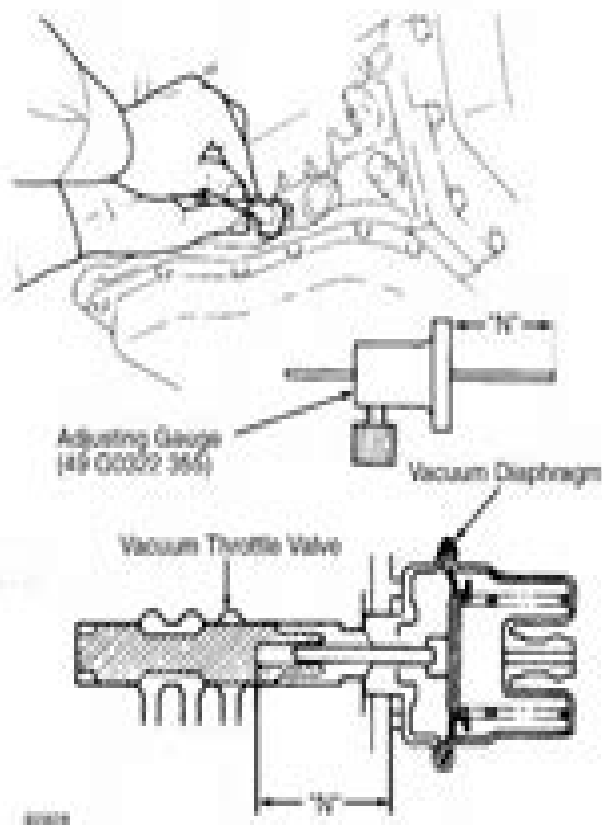
Fig. 4: Checking Vacuum Diaphragm Rod Length Courtesy of MAZDA MOTORS CORP.
