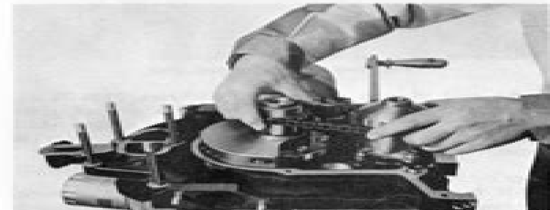
Fig. 1-79 Installing chain and sprockets
