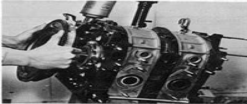
Fig. 1-76 Installing flywheel
