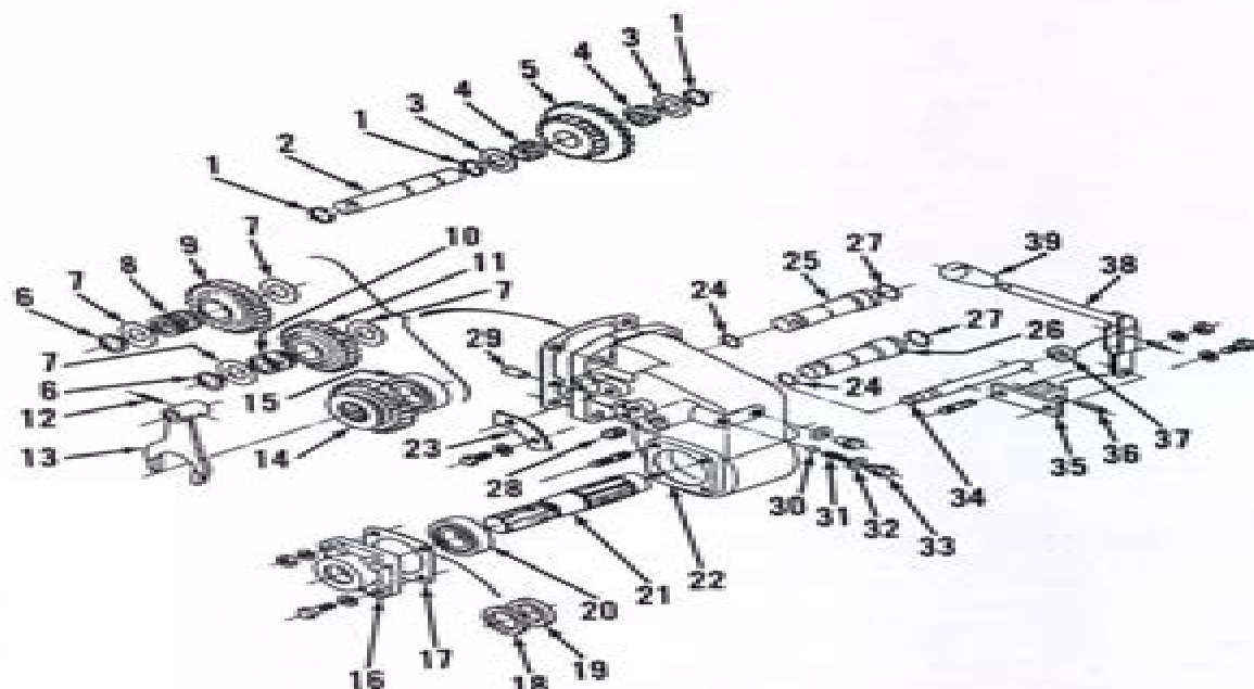
Fig. 6—Exploded view of transfer case assembly and associated components used on Model L225DT.
