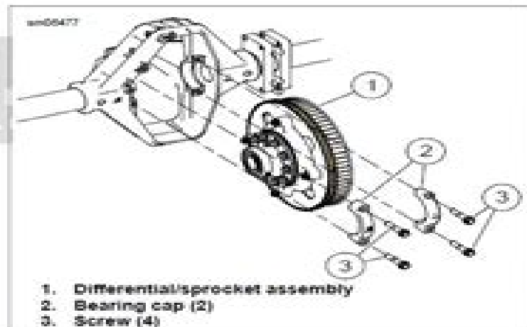
Figure 5-9. Differential and Sprocket Assembly
