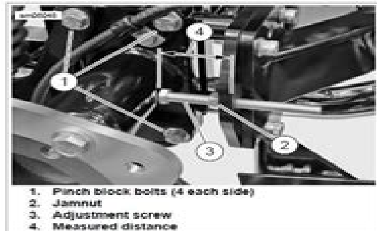
Figure 5-8. Adjust Axle
