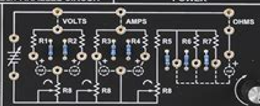
VOLTMETER/AMMETER/OHMMETER
