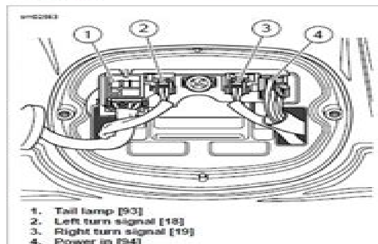
Figure 7-31. Wire Location at Connectors
