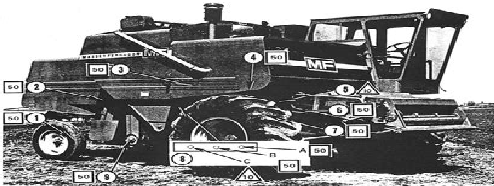
FIG. 103 — LUBRICATION — RIGHT-HAND SIDE
