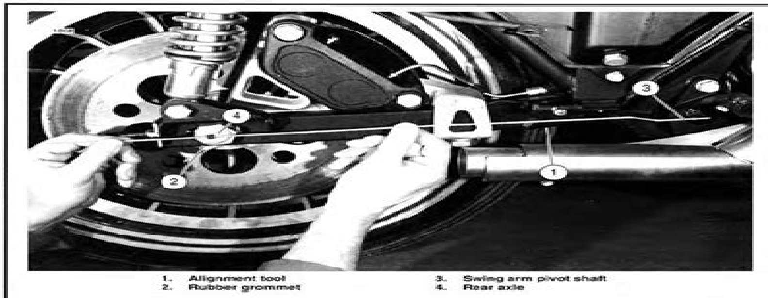
Figure 2-16. Measuring Rear Axle to Pivot Shaft Distance
