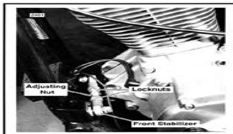
Figure 2-18. Adjusting Front Stabilizer
