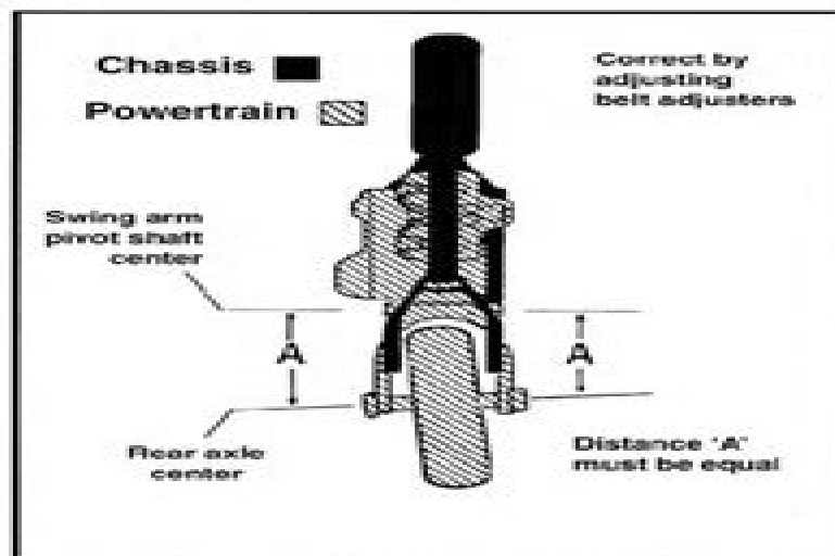
Figure 2-17. Rear Wheel Misaligned
