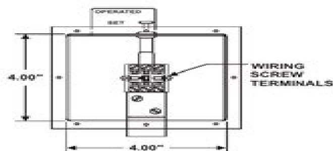
FRONT VIEW COVER REMOVED
