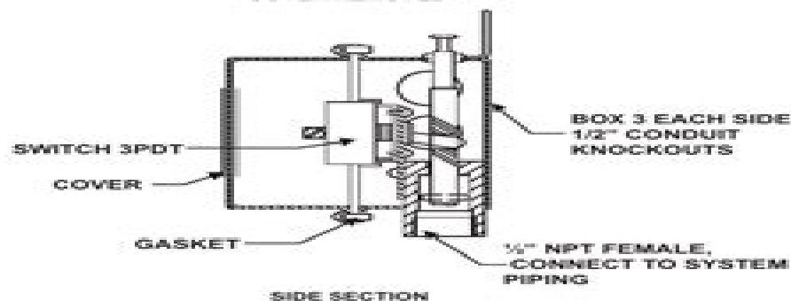
SIDE SECTION
