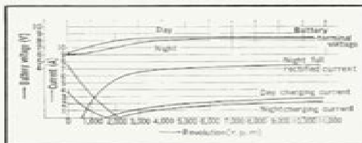
Figure 5-8. A.C. generator performance C50M, C65M
