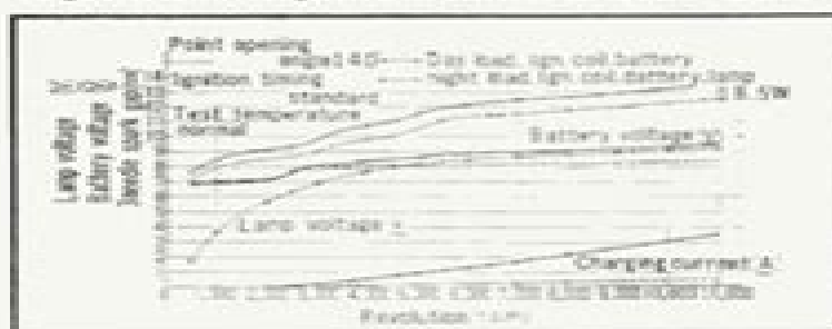
Figure 5-9. A.C. generator ignition coil performance
