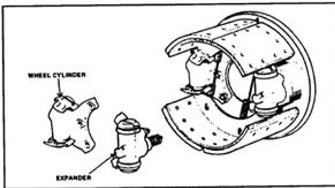
Lucas Girling A2LS Brake Assembly
