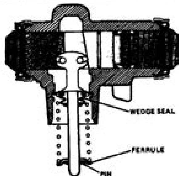
Expander Assy. Model Yr. 1984-1985
