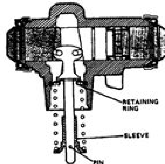
Expander Assy. Model Yr. 1986-Present
