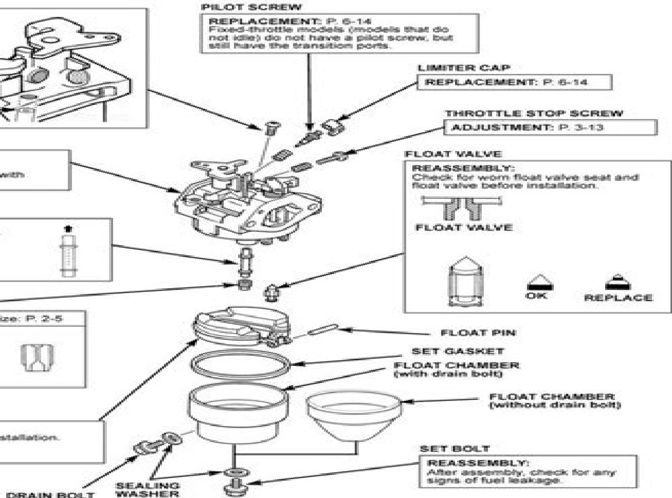
DRAIN BOLT
