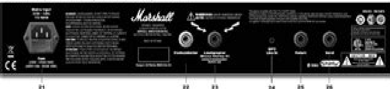
Rear panel shows MG50FX combo - MG100FX combo has the same features MG100FX head is identical except features two loudspeaker sockets
