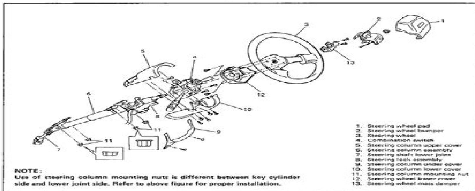
Fig. 3C-1 Steering Wheel and Column
